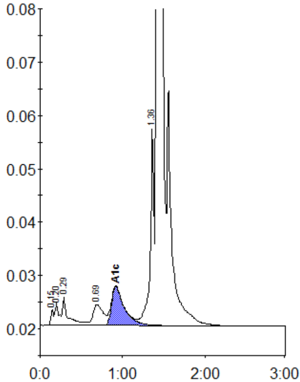
Peak table - ID: 10663383
